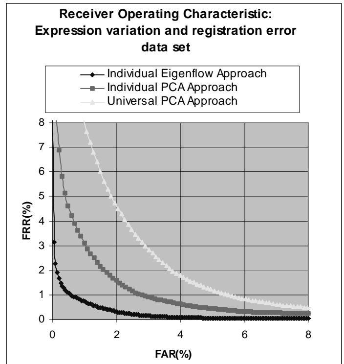
Figure 19 Experiment results on the data set containing both expression variations and registration errors.
