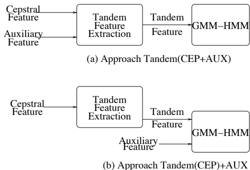
Figure 1: Illustration of the two approaches to incorporate auxiliary features in tandem systems
